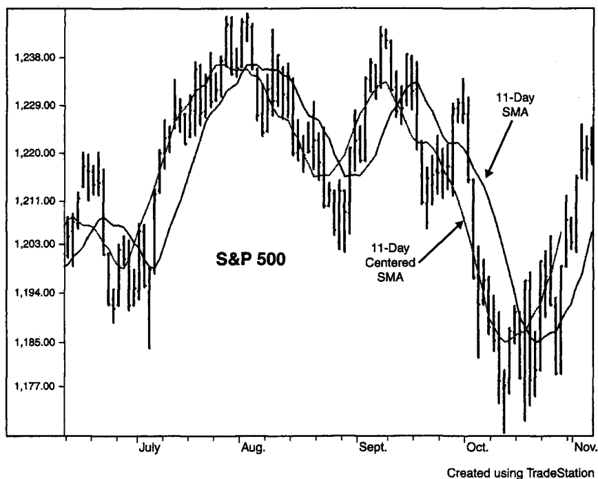
FIGURE 19.10 11-day centered moving average plot versus the standard moving average plot (daily: June 10, 2005-November 4, 2005)
