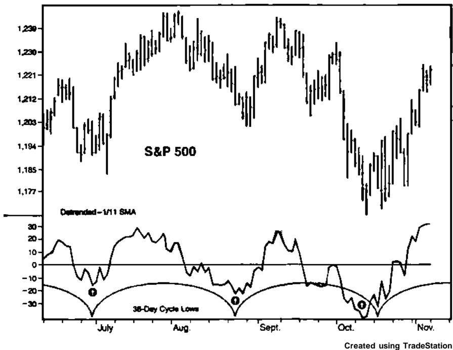
FIGURE 19.8 Detrended pic* 1- to 11-day SMA showing 38-day cycle lows [daily: June 10, 2005 - November 4, 2005)
