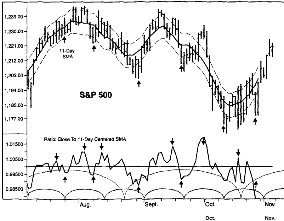
FIGURE 19.14 Ratio: Close to 1 1-day SMA showing short-term 14-day cycle highs and lows (daily: June 10, 2005-November 4, 2005)
