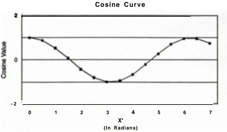
FIGURE 19.4 Plot of cosine curve
